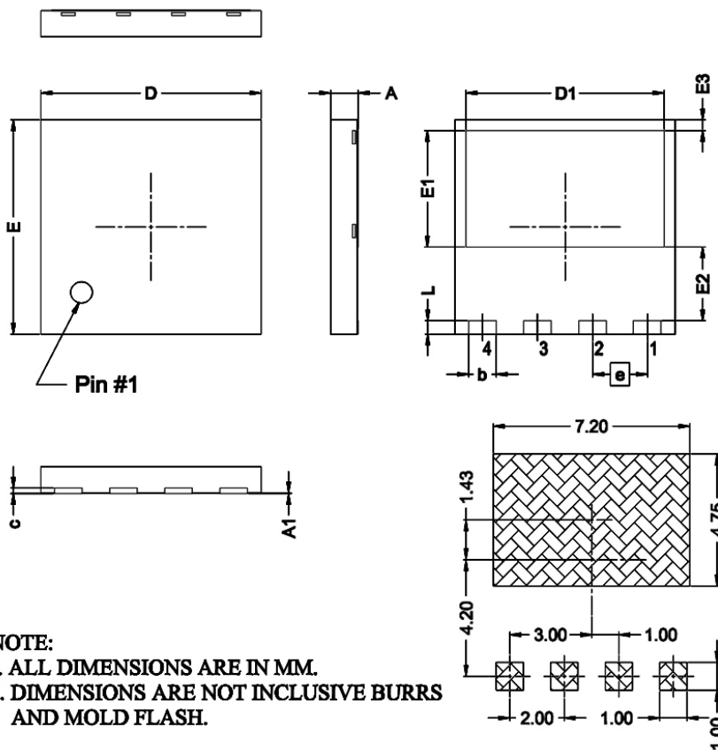
Land Pattern
